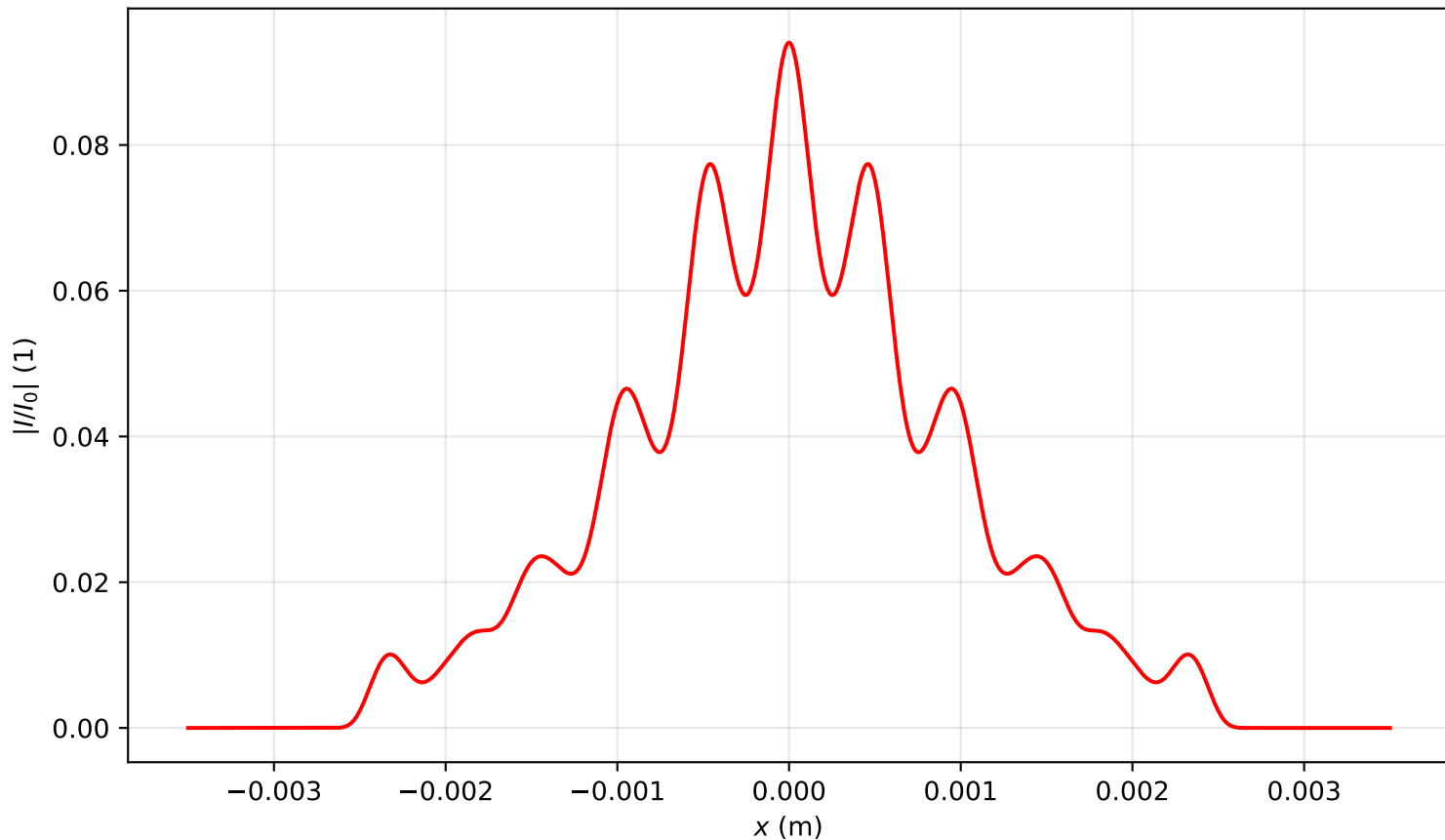
Intensity profile I(x, y = 0, z = 3.503)/I_0 , P_{in}=2.0P_{cr} , artificial time
